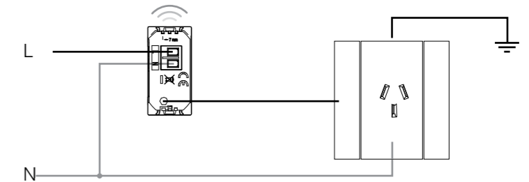
Wiring diagram
